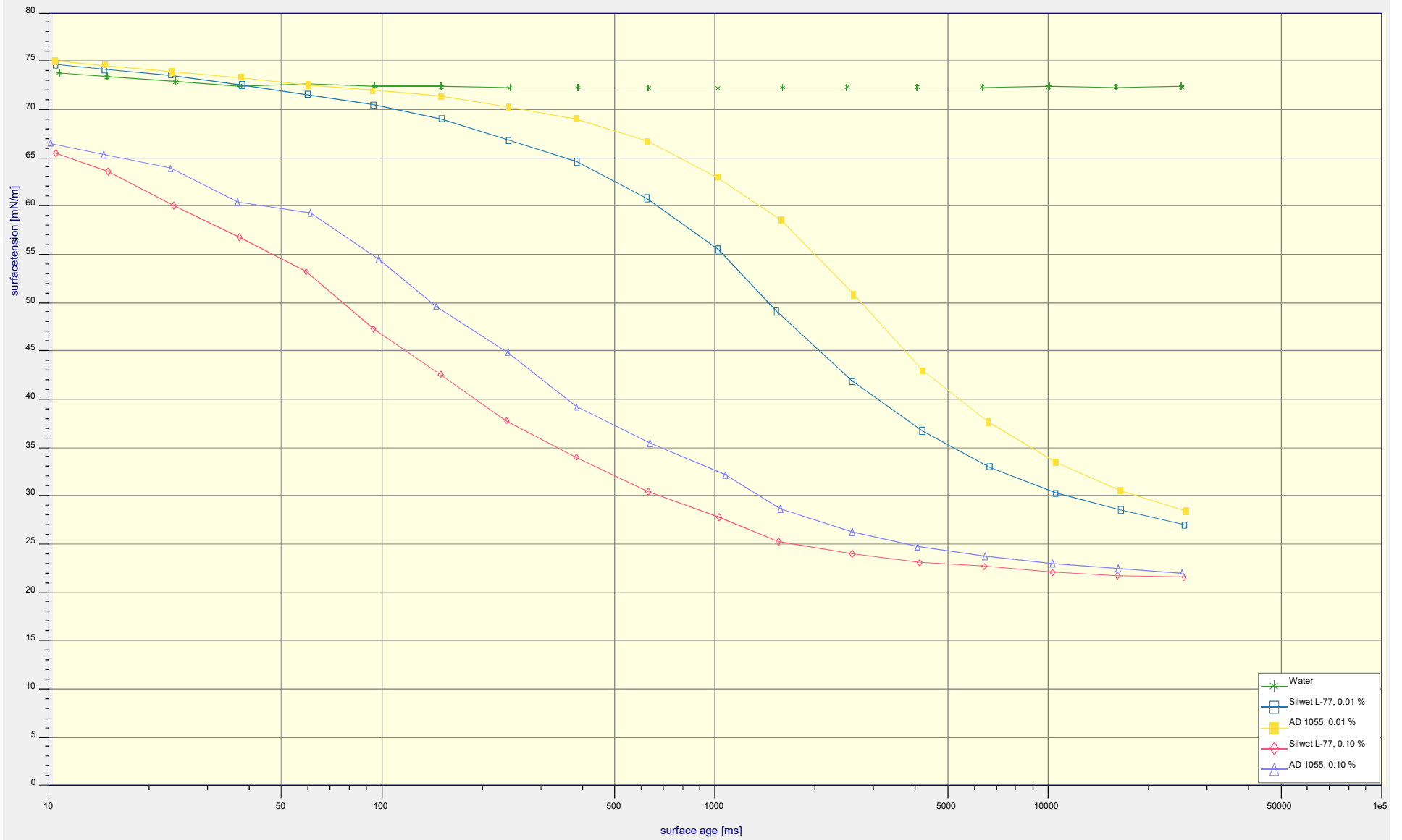
Surface tension vs. surface age
